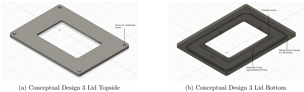
Figure 4.5: Conceptual Design 3 Lid
