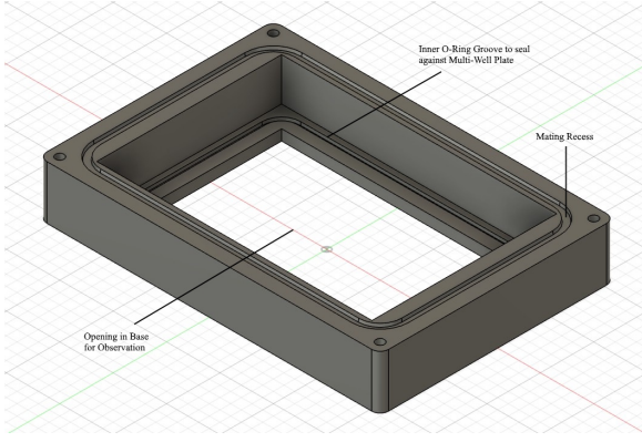
(a) Conceptual Design 2 Base
