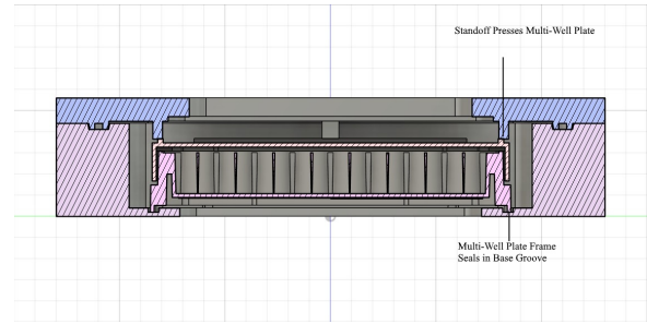
(b) Conceptual Design 3 Assembly
