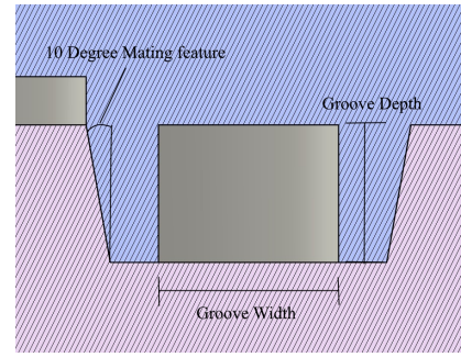
(b) Design 2 Mating Feature and O-ring Groove
