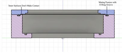
(a) Cross Section of Conceptual Design 2 Assembly
