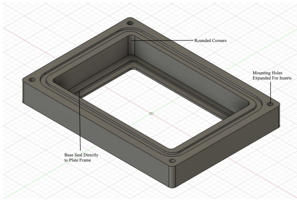
(a) Conceptual Design 3 Base
